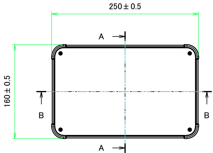
E view
